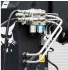
Hydraulic attachment lock
